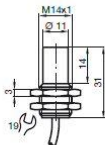
Sensor Pepperl + Fuchs NJ5 – 11 – N – G
